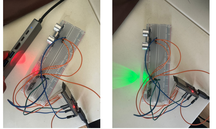
Fig. 4. The assembled prototype during testing.
